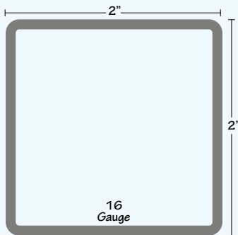
16GA/TRIPLE2X2 2" x 2" 16 gauge 24' Lengths
