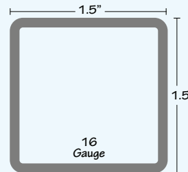
16GA/TPL1.5x1.5 1" x 2" 16 gauge 24' Lengths
