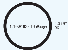
1315/24/TRIPLE 1.149" ID x 14 gauge 24' Lengths
