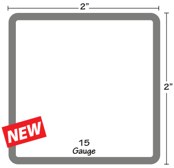
15GA/GATOR2x2 2" x 2" 15 gauge 24' Lengths
