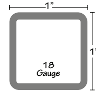
18GA/GATOR/24' 1" x 1" 18 gauge 24' Lengths
